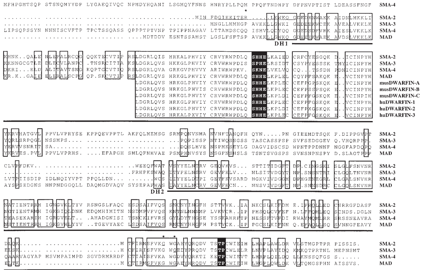
FIG. 3. Sequence of the dwarfins. Protein sequence alignment (40) of the dwarfin family. Dots represent gaps introduced to maximize alignments. Amino acids that are identical in more than half of the sequences shown are boxed. DH1 and DH2 are underlined. Amino acids altered in sma-2 and sma-3 alleles are identified by an asterisk and underlined. A short, highly conserved region of DH2 (GWGAEYQRQDVTS in SMA-2) appears to be an important mutational target, since one of two sma-2 , one of one sma-3 , and three of three Mad (38) alleles alter residues here. Putative Src homology 3-binding sites [PxxP (41)] are present in two each of the proteins, but these may be fortuitous, due to the proline-rich nature of the linkers. Two potential phosphorylation sites are conserved in this family (black boxes): a casein kinase II consensus [(S/T)xx(D/E) (42)] in DH1 and a mitogen-activated protein kinase (MAP kinase) minimal core site [(S/T)P (43)] in DH2. The GenBank accession numbers for the nematode sequences are U34778 ( sma-2 ), U34902 ( sma-3 ), and U34596 ( sma-4 ). mus, Mouse; hu, human.
