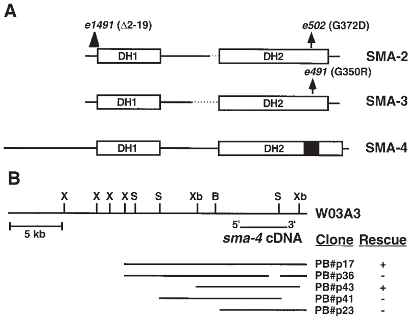
FIG. 2. Structure of sma-2 , sma-3 , and sma-4 . (A) Schematic protein structure of SMA-2, SMA-3, and SMA-4. Highly conserved regions (DH1 and DH2; see Fig. 3) are indicated by boxes. Amino acid deletions or changes are indicated in parentheses. (B) Transformation rescue to localize the gene sma-4 . The upper line represents a partial restriction map of the insert in the cosmid W03A3 that rescues the sma-4 Small and male tail phenotypes. Restriction sites: B, Bsi WI; S, Spe I; X, Xho I; Xb, Xba I. PB#p43 is a 10-kb Xba I fragment that rescues the sma-4 Small, but not the male tail, phenotype.
