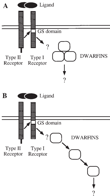
FIG. 4. Models for dwarffin action in TGF- \beta -like signaling. TGF- \beta -like receptors are heteromeric complexes of type I and type II transmembrane serine/threonine kinases. Type II receptors typically contain a short C-terminal extension on the intracellular domain. Type I receptors have a conserved motif, the GS domain, immediately upstream of the kinase domain, that is the site of phosphorylation by the type II receptor. We suggest that the dwarffins act downstream of TGF- \beta -like receptors in one of two possible ways. (A) The heteromeric complex model. (B) The sequential activation model.
