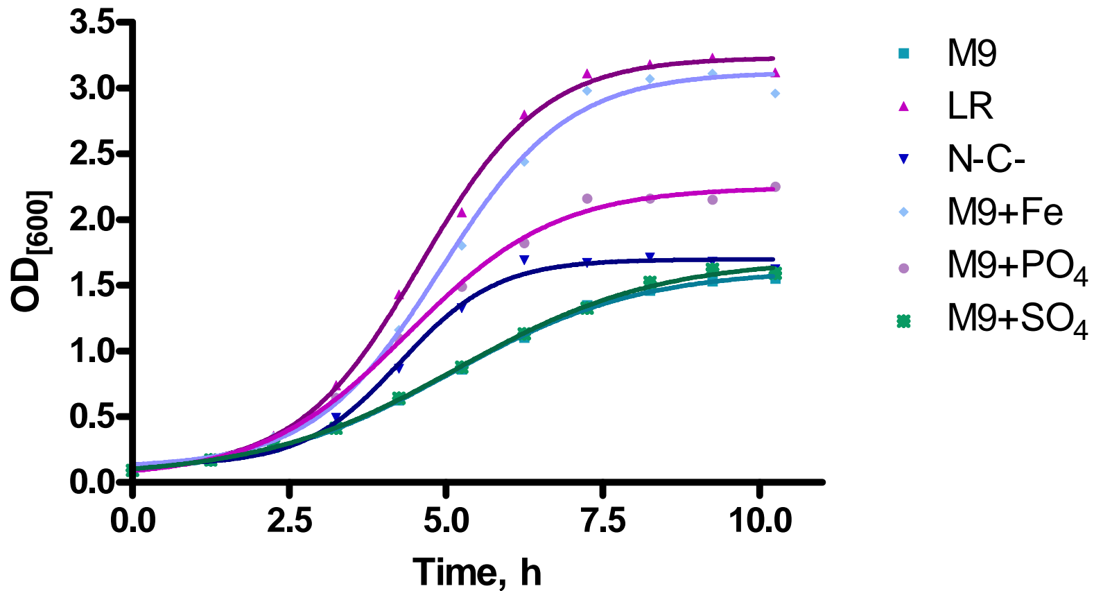
Growth curves of BL21 [DE3] on different minimal media
