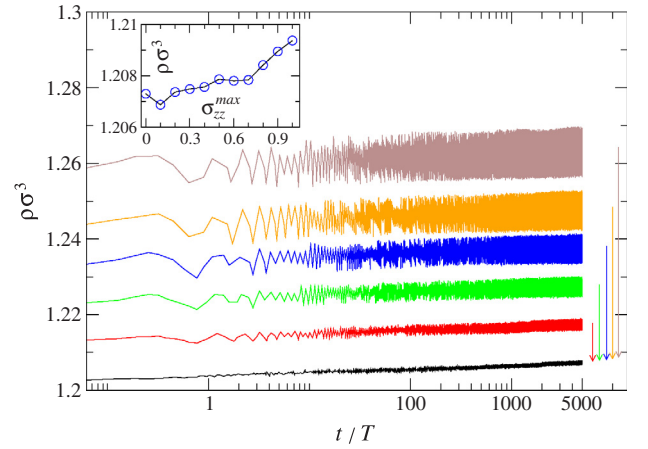
Fig. 4. The time dependence of the glass density, \rho\sigma^3 , during 5000 cycles for the stress amplitudes \sigma_{zz}^{max}\sigma^3/\varepsilon = 0.0, 0.2, 0.4, 0.6, 0.8, and 1.0 (from bottom to top). For clarity, the data are displaced vertically by +0.01\sigma^3 for \sigma_{zz}^{max} = 0.2\varepsilon\sigma^{-3} (red), by +0.02\sigma^3 for \sigma_{zz}^{max} = 0.4\varepsilon\sigma^{-3} (green), by +0.03\sigma^3 for \sigma_{zz}^{max} = 0.6\varepsilon\sigma^{-3} (blue), by +0.04\sigma^3 for \sigma_{zz}^{max} = 0.8\varepsilon\sigma^{-3} (orange), and by +0.055\sigma^3 for \sigma_{zz}^{max} = 1.0\varepsilon\sigma^{-3} (brown). The vertical displacements of the data are marked by the arrows. The inset shows the average glass density after 5000 cycles as a function of the stress amplitude (see text for details). (For interpretation of the references to color in this figure legend, the reader is referred to the web version of this article.)
