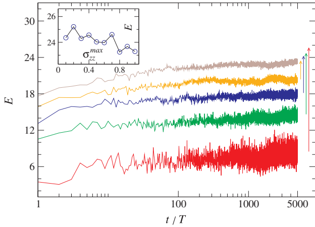
Fig. 5. The variation of the elastic modulus, E (in units of \varepsilon\sigma^{-3} ), during 5000 cycles for the stress amplitudes \sigma_{zz}^{max} \sigma^3/\varepsilon = 0.2, 0.4, 0.6, 0.8, and 1.0 (from bottom to top). The data are shifted by -17.0\varepsilon\sigma^{-3} for \sigma_{zz}^{max} \sigma^3/\varepsilon = 0.2 (red), by -10.0\varepsilon\sigma^{-3} for \sigma_{zz}^{max} \sigma^3/\varepsilon = 0.4 (green), by -6.0\varepsilon\sigma^{-3} for \sigma_{zz}^{max} \sigma^3/\varepsilon = 0.6 (blue), and by -3.0\varepsilon\sigma^{-3} for \sigma_{zz}^{max} \sigma^3/\varepsilon = 0.8 (orange). The offsets are indicated by the vertical arrows. The brown curve indicates the original data for \sigma_{zz}^{max} \sigma^3/\varepsilon = 1.0 . The inset shows E after 5000 cycles versus \sigma_{zz}^{max} . (For interpretation of the references to color in this figure legend, the reader is referred to the web version of this article.)
