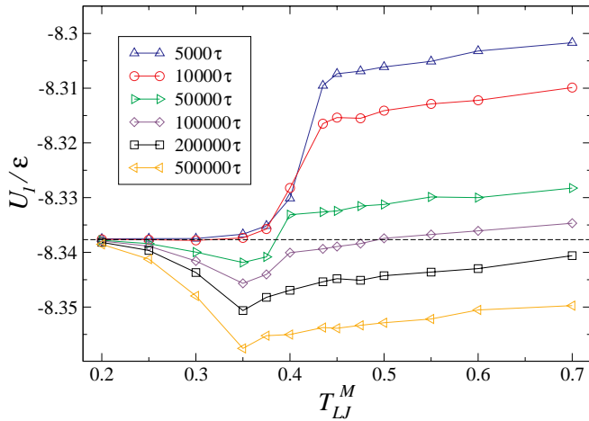
Fig. 6. The potential energy after the thermal cycle, U_1/\varepsilon , as a function of the thermal amplitude T_{LJ}^M (in units of \varepsilon/k_B ) for the oscillation periods T = 5000\tau ( \Delta ), 10000\tau ( \circ ), 50000\tau ( \triangleright ), 100000\tau ( \diamond ), 200000\tau ( \square ), and 500000\tau ( \triangleleft ). The horizontal dashed line denotes the potential energy level at the beginning of the thermal cycle.
