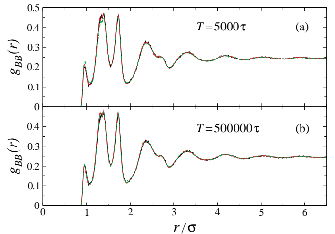
Fig. 7. The radial distribution function, g_{BB}(r) , for binary glasses at T_{LJ} = 0.01\varepsilon/k_B after thermal loading with periods (a) T = 5000\tau and (b) T = 500000\tau . The maximum temperatures of the thermal treatment are T_{LJ}^M = 0.35\varepsilon/k_B (solid red) and T_{LJ}^M = 0.70\varepsilon/k_B (dashed green). The data after the initial cooling with the rate 10^{-5}\varepsilon/k_B\tau are denoted by the solid black curves.
