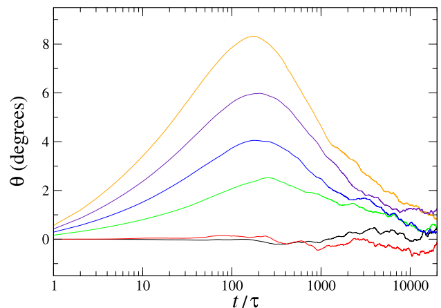
FIG. 7. The rotation angle along the displacement vector of the center of mass for the surface energies at both hemispheres (1.0 \varepsilon, 0.1 \varepsilon) , (1.0 \varepsilon, 0.3 \varepsilon) , (1.0 \varepsilon, 0.5 \varepsilon) , (1.0 \varepsilon, 0.7 \varepsilon) , and (1.0 \varepsilon, 1.0 \varepsilon) from top to bottom. The data for uniformly wetting (1.0 \varepsilon, 1.0 \varepsilon) and nonwetting (0.1 \varepsilon, 0.1 \varepsilon) particles are indicated by the black and red curves, respectively.
