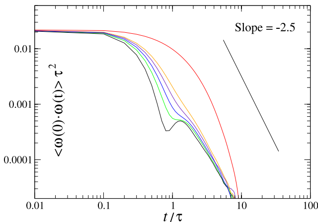
FIG. 6. The angular velocity autocorrelation function \langle \boldsymbol{\omega}(0) \cdot \boldsymbol{\omega}(t) \rangle for the LJ interaction energies at both hemispheres (0.1 \varepsilon, 0.1 \varepsilon) , (1.0 \varepsilon, 0.1 \varepsilon) , (1.0 \varepsilon, 0.3 \varepsilon) , (1.0 \varepsilon, 0.5 \varepsilon) , (1.0 \varepsilon, 0.7 \varepsilon) , and (1.0 \varepsilon, 1.0 \varepsilon) from top to bottom. The black line with a slope -2.5 is plotted for reference.
