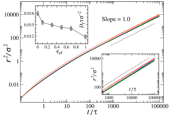
FIG. 3. The mean square displacement of particles as a function of time for the surface energies at both hemispheres from top to bottom (0.1\varepsilon, 0.1\varepsilon) , (1.0\varepsilon, 0.1\varepsilon) , (1.0\varepsilon, 0.3\varepsilon) , (1.0\varepsilon, 0.5\varepsilon) , (1.0\varepsilon, 0.7\varepsilon) , and (1.0\varepsilon, 1.0\varepsilon) . The dashed line with unit slope is plotted for reference. The lower inset shows an enlarged view of the same data at large times. The upper inset shows the diffusion coefficient as a function of \varepsilon_{\text{pf}} , while the other hemisphere is wetting, i.e., \varepsilon_{\text{pf}} = 1.0\varepsilon . The case \varepsilon_{\text{pf}} = 0 corresponds to a uniformly nonwetting particle (0.1\varepsilon, 0.1\varepsilon) .
