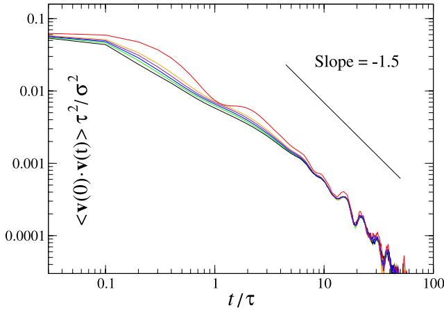
FIG. 5. The velocity autocorrelation function \langle \mathbf{v}(0) \cdot \mathbf{v}(t) \rangle for the interaction energies at both hemispheres (0.1 \varepsilon, 0.1 \varepsilon) , (1.0 \varepsilon, 0.1 \varepsilon) , (1.0 \varepsilon, 0.3 \varepsilon) , (1.0 \varepsilon, 0.5 \varepsilon) , (1.0 \varepsilon, 0.7 \varepsilon) , and (1.0 \varepsilon, 1.0 \varepsilon) from top to bottom. The straight line with a slope -1.5 is shown as a reference.
