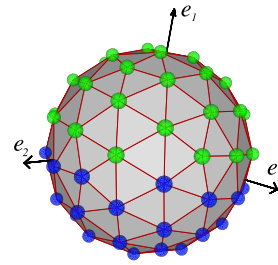
FIG. 1. A snapshot of the Janus particle with wetting (blue atoms) and nonwetting (green atoms) hemispheres. The particle consists of 72 atoms rigidly fixed on vertices of a convex polyhedron (see text for details). Note that particle atoms are not drawn to scale. The unit vectors \mathbf{e}_1 , \mathbf{e}_2 , and \mathbf{e}_3 form an orthonormal basis in a reference frame of the particle.
