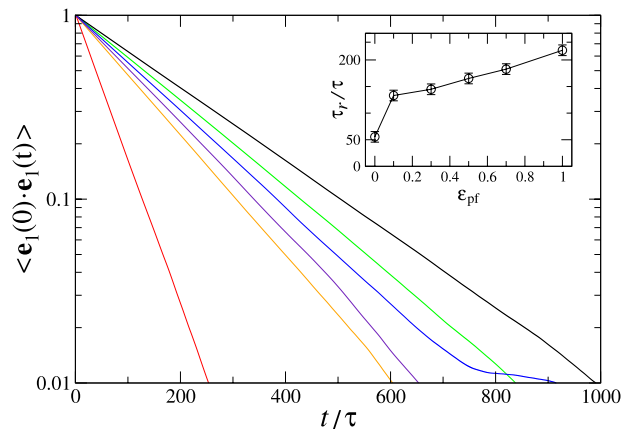
FIG. 4. The autocorrelation function \langle \mathbf{e}_1(0) \cdot \mathbf{e}_1(t) \rangle for the surface energies at both hemispheres (0.1\varepsilon, 0.1\varepsilon) , (1.0\varepsilon, 0.1\varepsilon) , (1.0\varepsilon, 0.3\varepsilon) , (1.0\varepsilon, 0.5\varepsilon) , (1.0\varepsilon, 0.7\varepsilon) , and (1.0\varepsilon, 1.0\varepsilon) from left to right. The inset shows the rotational relaxation time \tau_r (in units of \tau ) as a function of the surface energy at the nonwetting hemisphere.
