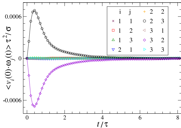
FIG. 8. The translational times angular velocity correlation functions \langle v_i(0) \cdot \omega_j(t) \rangle for the indicated pairs of indices. The velocity components are computed along the unit vectors \mathbf{e}_i (see Fig. 1). The data are reported for a Janus particle with the LJ interaction energies at both hemispheres ( 1.0 \epsilon , 0.1 \epsilon ).
