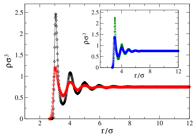
FIG. 2. Averaged fluid density profiles as a function of the distance from the particle center for uniformly wetting ( \diamond ) and uniformly nonwetting ( \nabla ) particles. The LJ interaction energy between particle atoms and fluid monomers is \varepsilon_{pf} = 1.0\varepsilon ( \diamond ) and \varepsilon_{pf} = 0.1\varepsilon ( \nabla ). The inset shows fluid density profiles near the wetting hemisphere \varepsilon_{pf} = 1.0\varepsilon ( \times ) and nonwetting hemisphere \varepsilon_{pf} = 0.1\varepsilon ( \circ ) of the Janus particle.
