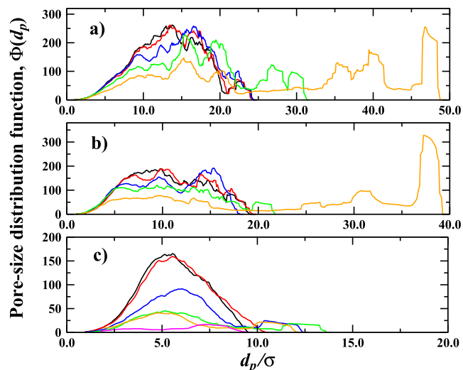
Fig. 9. The pore size distribution functions for three samples strained after the waiting time of 5 \times 10^4 \tau . The colorcode for different curves is black ( \epsilon_{xx} = 0.0 ), red ( \epsilon_{xx} = 0.05 ), blue ( \epsilon_{xx} = 0.20 ), green ( \epsilon_{xx} = 0.40 ), orange ( \epsilon_{xx} = 0.80 ), and magenta ( \epsilon_{xx} = 1.60 ). The atomic configurations shown in Figs. 6–8 are described by the pore size distributions presented in the panels (a), (b), and (c), respectively.
