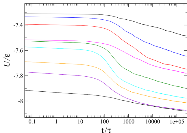
Fig. 3. The time dependence of the potential energy per atom for nine samples at constant pressure P = 0 and T = 0.05\epsilon/k_B . The average glass density increases from top to bottom. The same samples and color codes as in Fig. 2.
