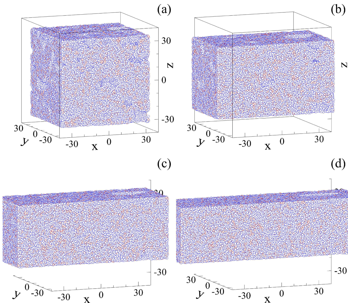
Fig. 8. Selected snapshots of the porous glass for strains and average glass densities (a) \epsilon_{xx} = 0.05 and \rho\sigma^3 = 1.0 , (b) \epsilon_{xx} = 0.40 and \rho\sigma^3 = 1.11 , (c) \epsilon_{xx} = 0.80 and \rho\sigma^3 = 1.16 , and (d) \epsilon_{xx} = 1.60 and \rho\sigma^3 = 1.18 . The stress dependence on strain is indicated by the cyan curve in Fig. 5.
