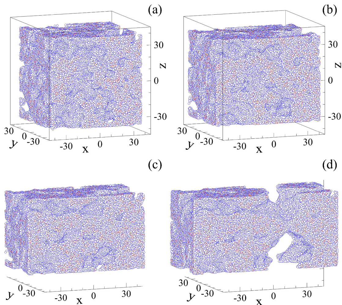
Fig. 7. Instantaneous snapshots for the values of strain and the average glass density (a) \epsilon_{xx} = 0.05 and \rho\sigma^3 = 0.69 , (b) \epsilon_{xx} = 0.20 and \rho\sigma^3 = 0.73 , (c) \epsilon_{xx} = 0.40 and \rho\sigma^3 = 0.80 , and (d) \epsilon_{xx} = 0.70 and \rho\sigma^3 = 0.70 . The stress is denoted by the magenta curve in Fig. 5.
