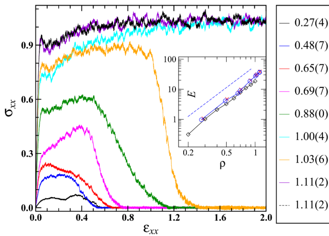
Fig. 5. The variation of stress \sigma_{xx} (in units of \epsilon\sigma^{-3} ) as a function of strain during tensile loading at zero pressure with the strain rate \dot{\epsilon}_{xx} = 10^{-4}\tau^{-1} . The samples with different average glass densities were strained after the waiting time of 5 \times 10^4\tau (see text for details). The values of the average glass density at zero strain are indicated in the legend. In the last two cases, the difference between measured average densities is beyond the precision. The inset shows the elastic modulus E (in units of \epsilon\sigma^{-3} ) as a function of the average glass density \rho\sigma^3 . The data in the inset were computed after the waiting time of 5 \times 10^4\tau (blue circles) and after 15 \times 10^4\tau (red crosses). For reference, the data for the elastic modulus at constant volume (taken from Ref. [17]) are also shown by black diamonds. The straight dashed line indicates the slope of 2.41.
