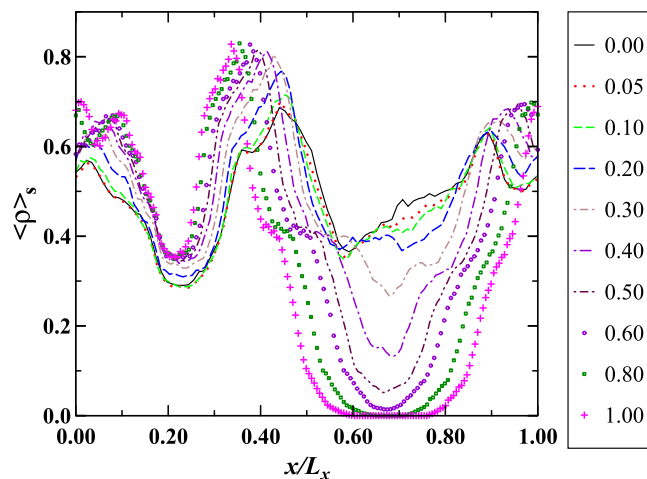
Fig. 10. The averaged density profiles \langle \rho \rangle_s(x) (in units of \sigma^{-3} ) computed along the x -axis (corresponding to the loading direction), are plotted for different values of the applied strain, as shown in the figure legend. The system snapshots are presented in Fig. 6 for four values of strain.
