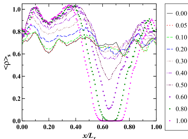
Fig. 11. The local density profiles \langle \rho \rangle_s(x) (in units of \sigma^{-3} ) along the loading direction are presented for the indicated values of strain. Atomic configurations for this sample are shown in Fig. 7 for selected values of strain.
