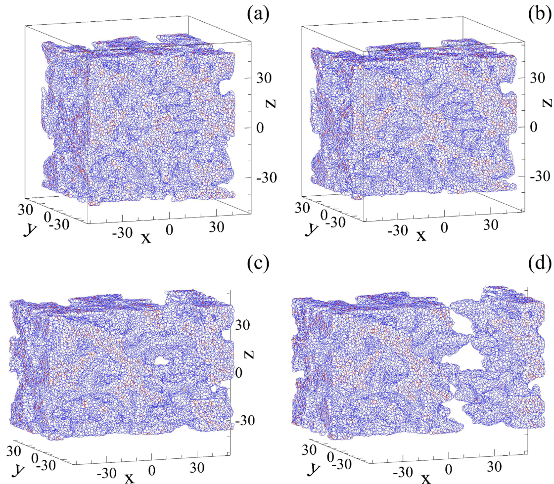
Fig. 6. Atomic configurations of the strained porous glass at zero pressure and temperature T = 0.05\epsilon/k_B . The values of strain and the average glass density are (a) \epsilon_{xx} = 0.05 and \rho\sigma^3 = 0.48 , (b) \epsilon_{xx} = 0.20 and \rho\sigma^3 = 0.49 , (c) \epsilon_{xx} = 0.40 and \rho\sigma^3 = 0.47 , and (d) \epsilon_{xx} = 0.60 and \rho\sigma^3 = 0.41 . The strain rate is \dot{\epsilon}_{xx} = 10^{-4}\tau^{-1} . The stress-strain curve for this sample is marked by blue color in Fig. 5.
