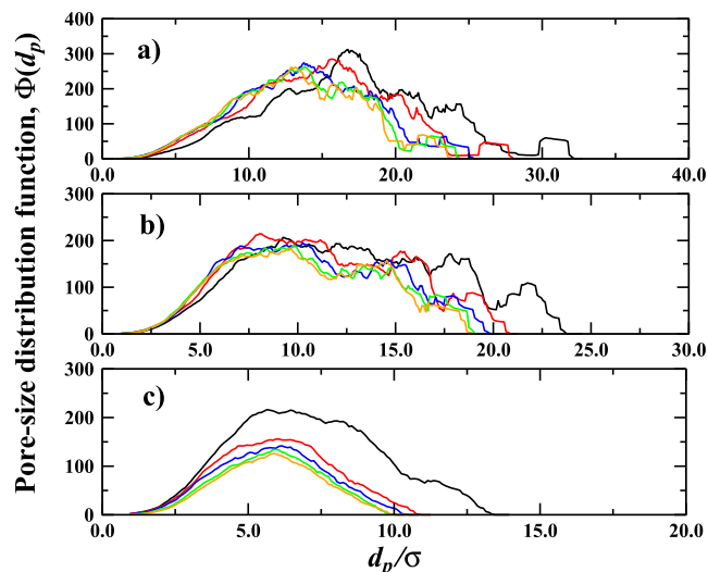
Fig. 4. The pore size distributions in quiescent samples during the structural relaxation process at constant pressure. The average glass densities at t = 0 are (a) \rho\sigma^3 = 0.3 , (b) \rho\sigma^3 = 0.5 , and (c) \rho\sigma^3 = 0.8 . The distribution functions for different waiting times are indicated by black curves ( t = 0 ), red curves ( t = 5 \times 10^2\tau ), blue curves ( t = 5 \times 10^3\tau ), green curves ( t = 5 \times 10^4\tau ), and orange curves ( t = 2.5 \times 10^5\tau ). Note that scales are different in three panels.
