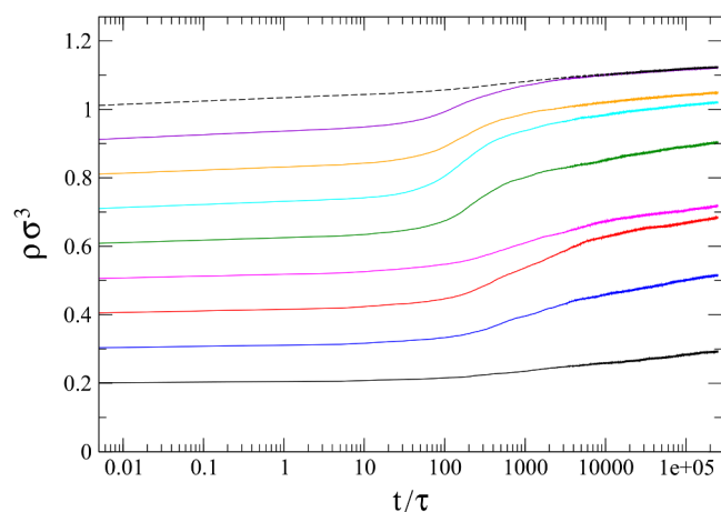
Fig. 2. The average glass densities as a function of waiting time during the aging process at zero pressure and temperature T = 0.05\epsilon/k_B . The average density of porous samples at t = 0 is \rho\sigma^3 = 0.2, 0.3, 0.4, 0.5, 0.6, 0.7, 0.8, 0.9 , and 1.0 (from bottom to top).
