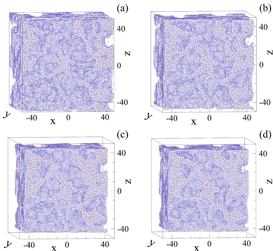
Fig. 1. A series of snapshots of the porous glass at zero pressure after time intervals (a) 0\tau , (b) 500\tau , (c) 50000\tau , and (d) 250000\tau . The average glass densities are (a) \rho\sigma^3 = 0.30 , (b) \rho\sigma^3 = 0.37 , (c) \rho\sigma^3 = 0.49 , and (d) \rho\sigma^3 = 0.52 . The temperature is T = 0.05\epsilon/k_B and the total number of atoms is N = 300000 . Atoms of types A and B are denoted by blue and red spheres. Note that the size of atoms is reduced for clarity.
