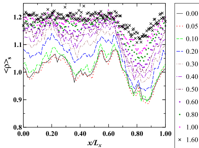
Fig. 12. The density profiles \langle \rho \rangle_s(x) (in units of \sigma^{-3} ) are plotted for the values of strain listed in the legend. The corresponding atomic configurations are displayed in Fig. 8 for selected values of strain.
