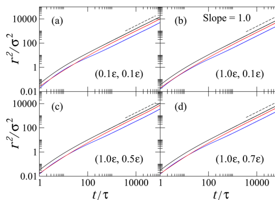
Figure 7. Averaged mean square displacements in the direction parallel (blue curves) and perpendicular (red curves) to the main axis of (a) a uniformly nonwetting particle with \epsilon_{pf} = 0.1\epsilon and Janus particles with surface energies (b) (1.0\epsilon, 0.1\epsilon) , (c) (1.0\epsilon, 0.5\epsilon) , and (d) (1.0\epsilon, 0.7\epsilon) . The total mean square displacement is indicated by black curves. The dashed lines show unit slope.
