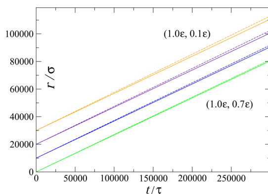
Figure 8. Total displacement, r/\sigma , of the centers of nonwetting (dashed lines) and wetting (solid lines) ends of Janus particles with surface energies (1.0\epsilon, 0.1\epsilon) , (1.0\epsilon, 0.3\epsilon) , (1.0\epsilon, 0.5\epsilon) , and (1.0\epsilon, 0.7\epsilon) from top to bottom. The data for the first three cases are displaced vertically for clarity.
